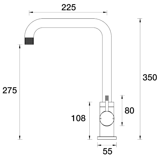
Elm Sink 90 Degree Mixer A40.025.1.01 - Chrome
