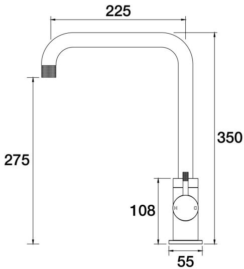
Elm Sink 90 Degree Mixer A40.025.1.57 - Matt Nickel
