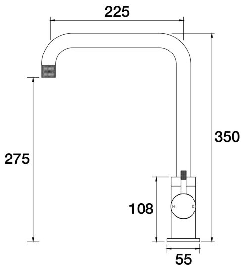
Elm Sink 90 Degree Mixer A40.025.1.67 - Vintage Brass
