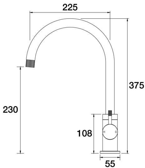
Elm Sink Gooseneck Mixer A40.026.1.54 - Volcanic Grey
