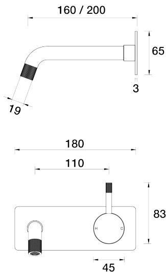
Elm Wall Mixer Basin Set 160mm outlet Incl. plate A40.032.1.01 - Chrome
