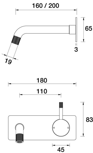
Elm Wall Mixer Basin Set on plate 160mm A40.032.1.01 - Chrome
