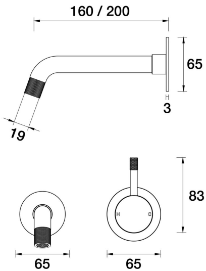
Elm Wall Mixer Basin Set 160mm outlet A40.032.2.01 - Chrome
