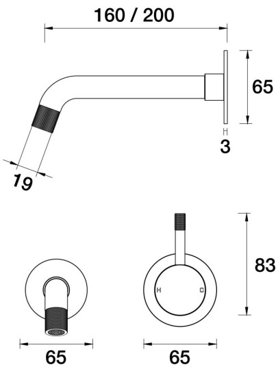
Elm Wall Mixer Basin Set 160mm outlet A40.032.2.01 - Chrome
