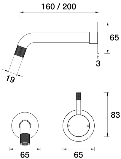
Elm Wall Mixer Basin Set 160mm outlet A40.032.2.52 - Burnished
