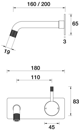
Elm Wall Mixer Basin Set on plate 200mm A40.032.3.01 - Chrome
