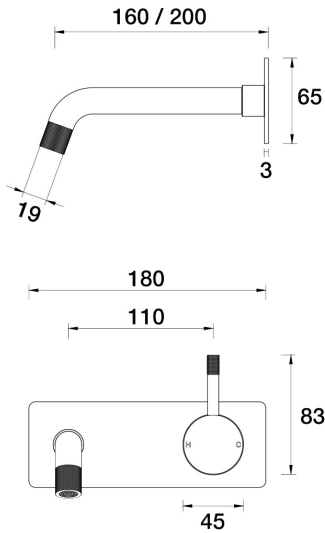
Elm Wall Mixer Basin Set 200mm outlet Incl. plate A40.032.3.24 - Brushed Gunmetal
