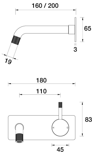
Elm Wall Bath Mixer Set 160mm outlet Incl. plate A40.041.1.45 - Native Brass
