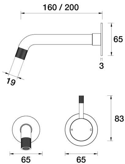
Elm Wall Bath Mixer Set 160mm outlet A40.041.2.67 - Vintage Brass
