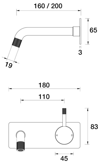
Elm Wall Bath Mixer Set 200mm outlet Incl. plate A40.041.3.52 - Burnished
