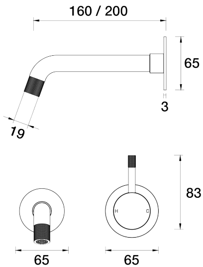
Elm Wall Bath Mixer Set 200mm outlet A40.041.4.01 - Chrome
