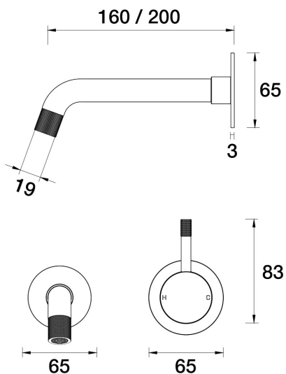
Elm Wall Bath Mixer Set 200mm outlet A40.041.4.25 - Brushed Nickel
