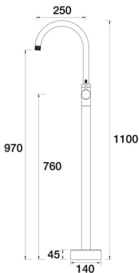
Elm Floor Bath Filler Mixer - Gooseneck A40.072.1.23 - Gunmetal
