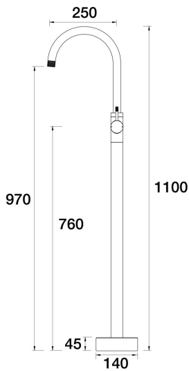
Elm Floor Bath Filler Mixer - Gooseneck A40.072.1.48 - Copper
