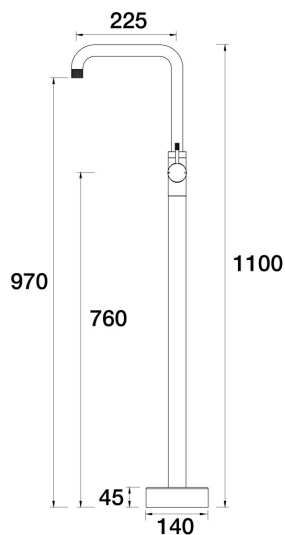
Elm Floor Bath Filler Mixer - 90 Degree A40.073.1.21 - Brushed Rose Gold
