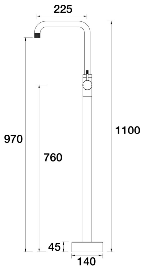
Elm Floor Bath Filler Mixer - 90 Degree A40.073.1.40 - Rumbled Brass
