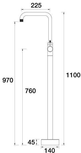
Elm Floor Bath Filler Mixer - 90 Degree A40.073.1.48 - Copper
