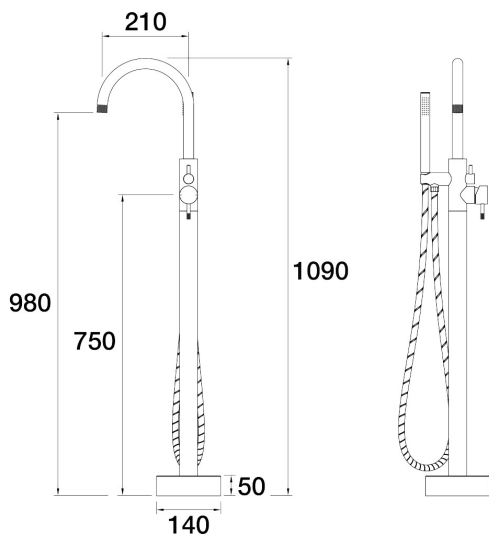
Elm Floor Bath Filler Mixer with Handshower Gooseneck A40.075.1.39 - Antique Bronze
