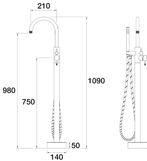
Elm Floor Bath Filler Mixer with Handshower Gooseneck A40.075.1.67 - Vintage Brass
