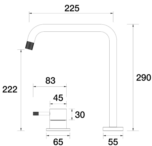
Elm Hob Mixer Set A40.081.2.23 - Gunmetal
