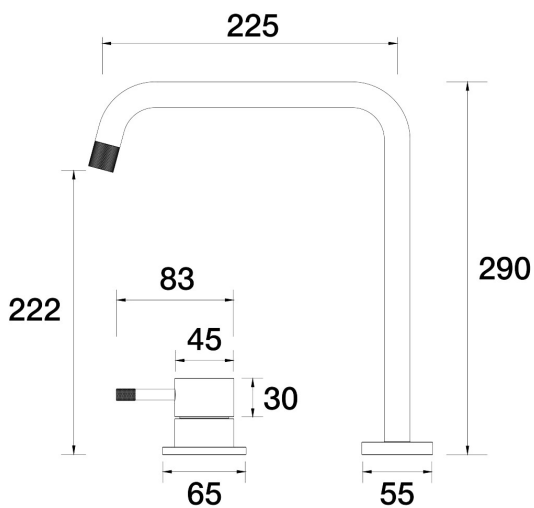
Elm Hob Mixer Set A40.081.2.34 - Matt Black
