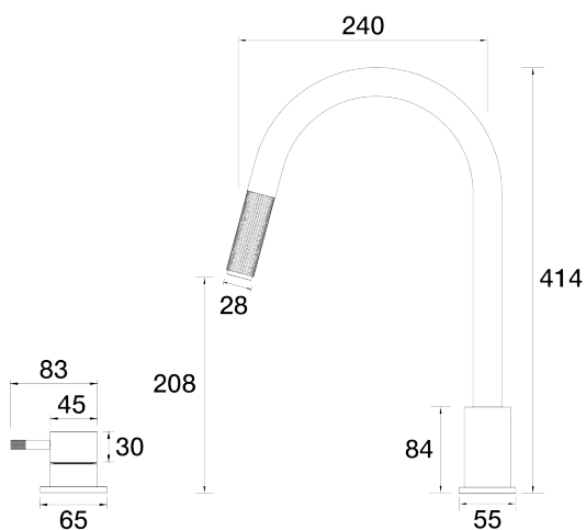
Elm Hob Mixer Pullout Gooseneck Set A40.081.3.01 - Chrome
