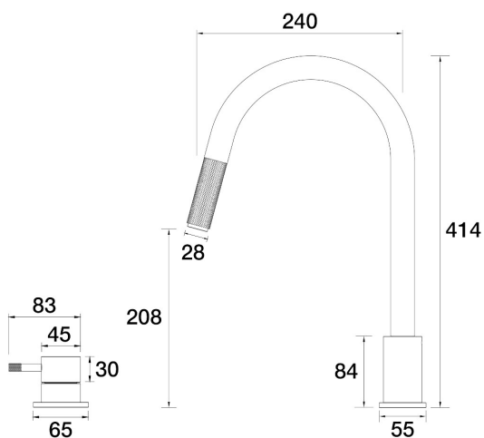
Elm Hob Mixer Pullout Gooseneck Set A40.081.3.21 - Brushed Rose Gold
