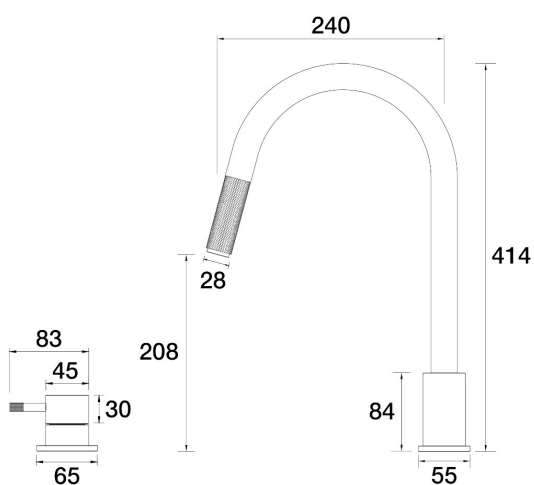
Elm Hob Mixer Pullout Gooseneck Set A40.081.3.25 - Brushed Nickel
