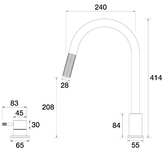
Elm Hob Mixer Pullout Gooseneck Set A40.081.3.44 - Antique Copper
