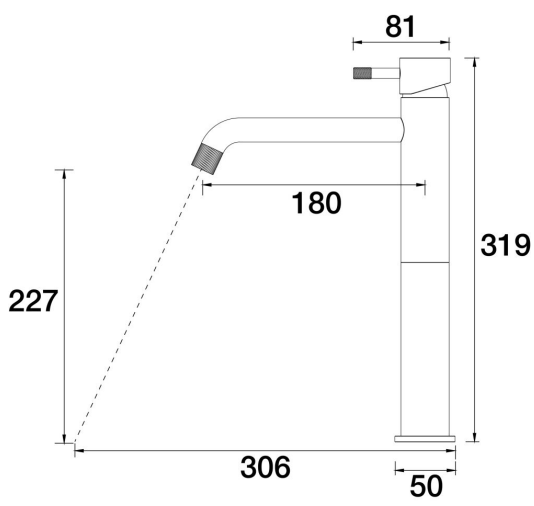
Elm Cable Hob Basin Tower Mixer A41.012.1.01 - Chrome
