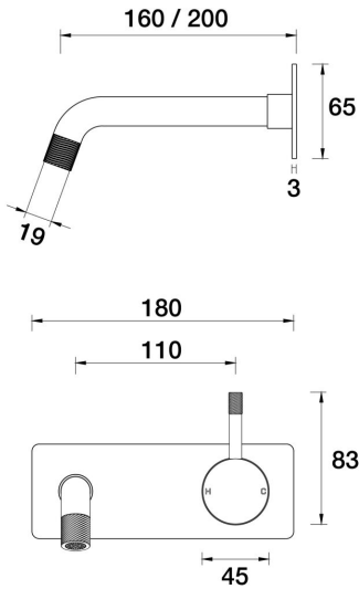
Elm Cable Wall Mixer Basin Set on plate 160mm A41.032.1.01 - Chrome
