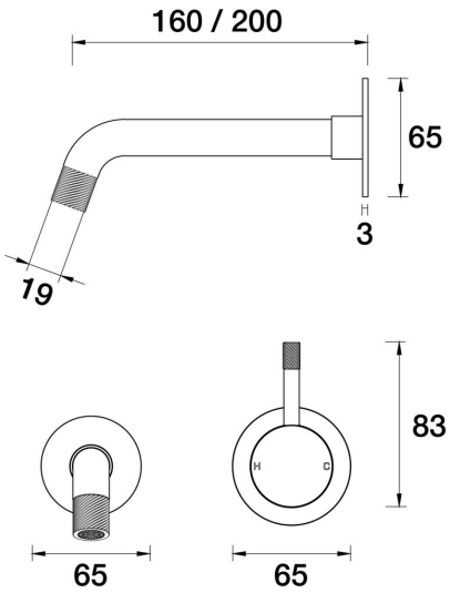
Elm Cable Wall Mixer Basin Set 160mm outlet A41.032.2.01 - Chrome
