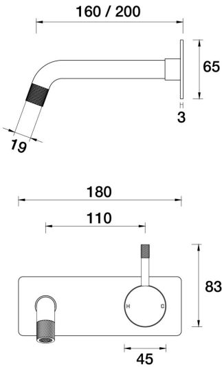
Elm Cable Wall Mixer Basin Set on plate 200mm A41.032.3.01 - Chrome
