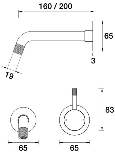
Elm Cable Wall Bath Mixer Set 200mm outlet A41.041.4.01 - Chrome
