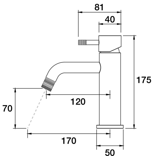
Elm Lane Hob Basin Mixer A42.011.2.39 - Antique Bronze
