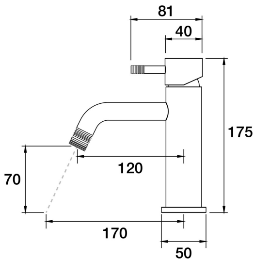
Elm Lane Hob Basin Mixer A42.011.2.45 - Native Brass
