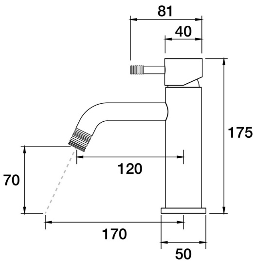
Elm Lane Hob Basin Mixer A42.011.2.67 - Vintage Brass
