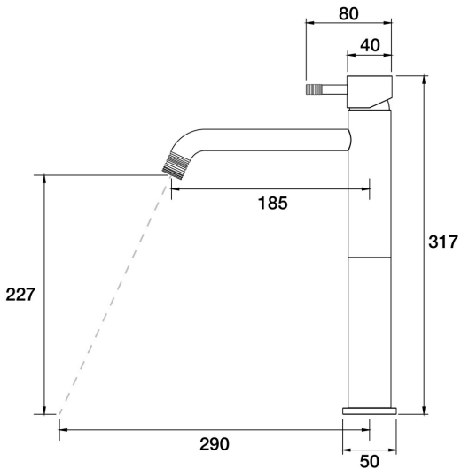
Elm Lane Hob Basin Tower Mixer A42.012.1.32 - Midnight Black
