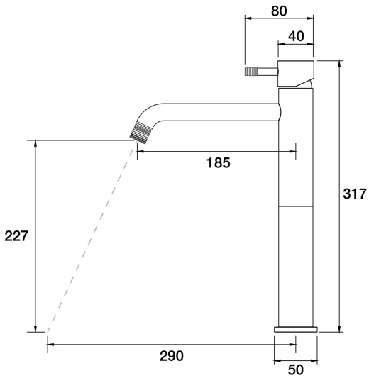
Elm Lane Hob Basin Tower Mixer A42.012.1.40 - Rumbled Brass
