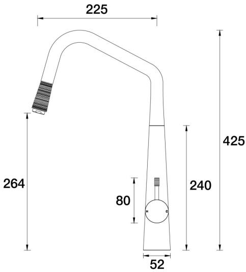
Elm Lane Sink Pull-Out Mixer A42.024.1.01 - Chrome
