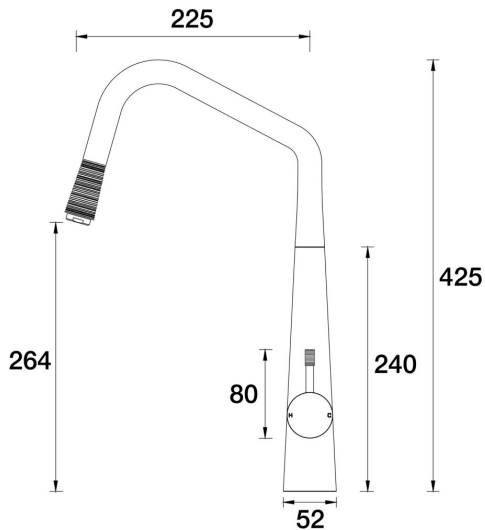
Elm Lane Sink Pull-Out Mixer A42.024.1.40 - Rumbled Brass
