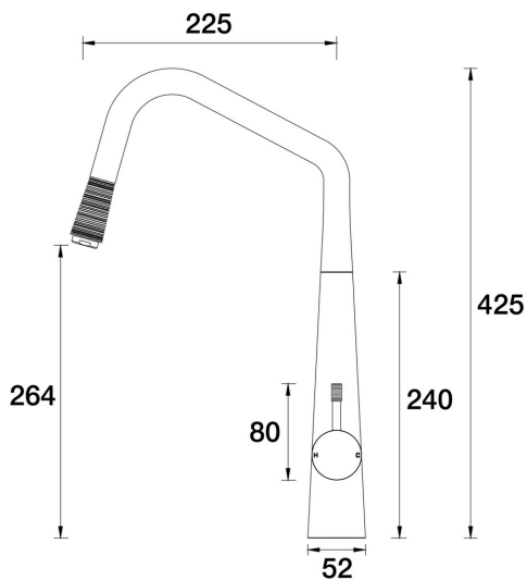
Elm Lane Sink Pull-Out Mixer A42.024.1.41 - Brushed Brass
