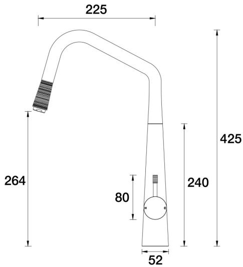
Elm Lane Sink Pull-Out Mixer A42.024.1.45 - Native Brass
