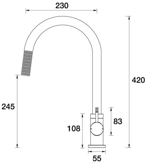
Elm Lane Sink Pull-Out Mixer Gooseneck A42.024.2.01 - Chrome
