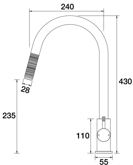
Elm Lane Sink Pull-Out Mixer Gooseneck A42.024.2.48 - Copper
