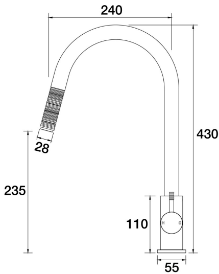
Elm Lane Sink Pull-Out Mixer Gooseneck A42.024.2.54 - Volcanic Grey
