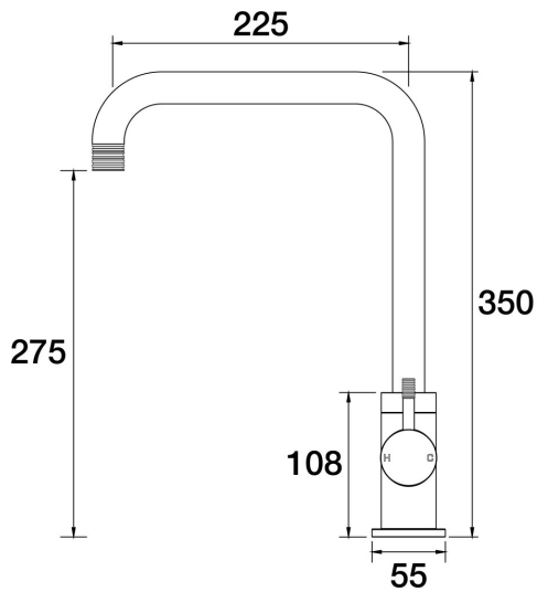
Elm Lane Sink 90 Degree Mixer A42.025.1.43 - Brass
