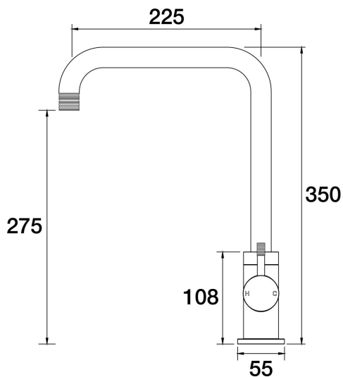
Elm Lane Sink 90 Degree Mixer A42.025.1.57 - Matt Nickel
