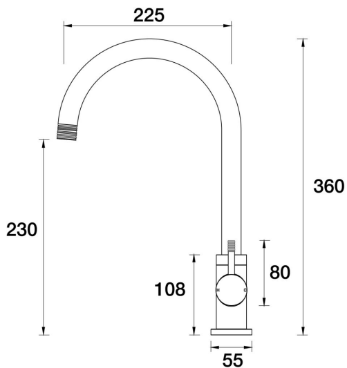
Elm Lane Sink Gooseneck Mixer A42.026.1.01 - Chrome
