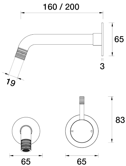
Elm Lane Wall Mixer Basin Set 200mm outlet A42.032.4.01 - Chrome
